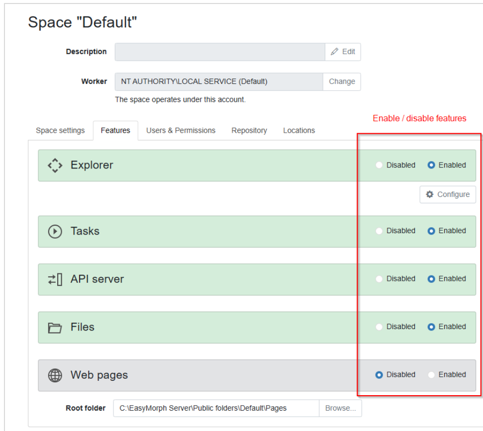
Screenshot 13: Enabling/disabling space features.
