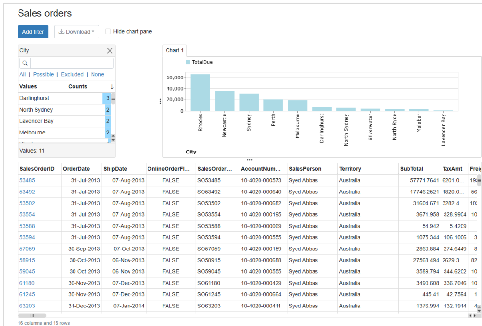
Screenshot 17: Analysis View of a computed dataset.
