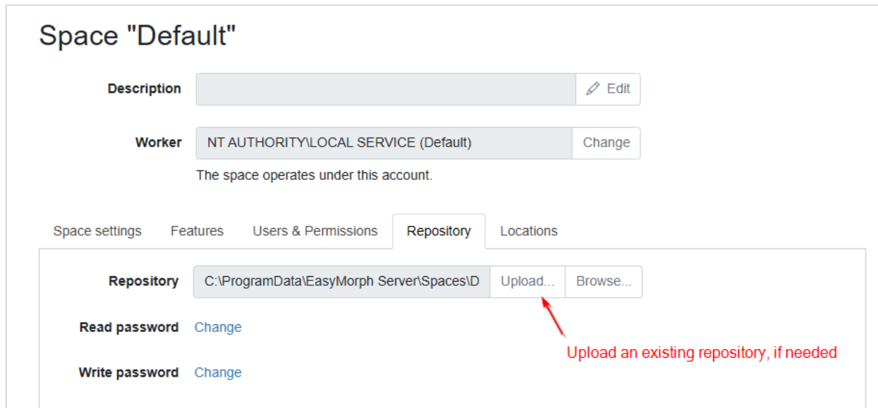
Screenshot 7: Connector repository configuration in space settings.
