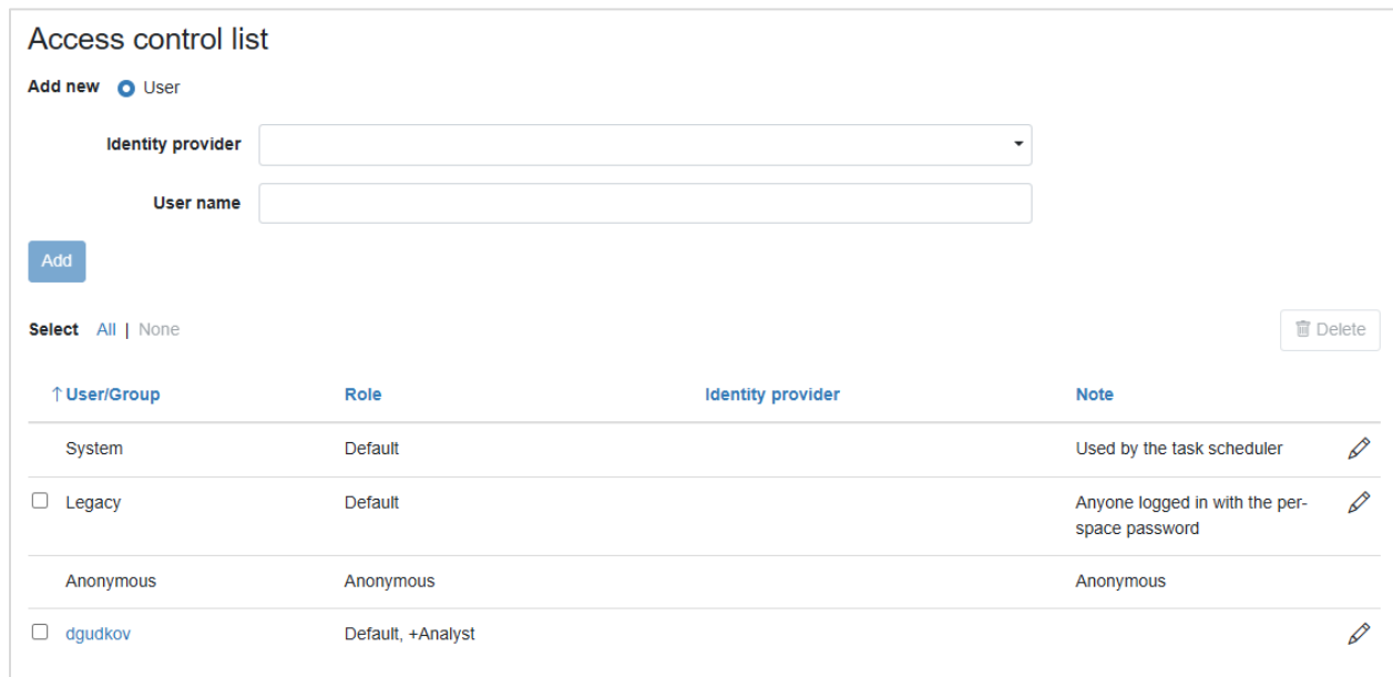
Screenshot 12: Access control list of a space.
